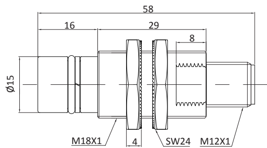
Fig. 2 Inductive sensor with M12 connector (flush)
