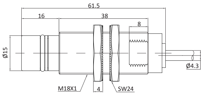
Fig. 1 Inductive sensor with cable (flush)
